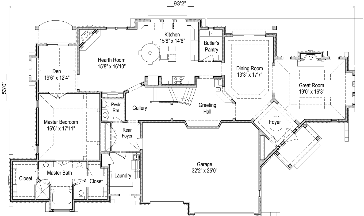
First Floor Plan: 2833 sq. ft.
